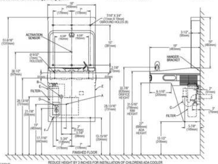
WaterSentry® Plus Filter System
