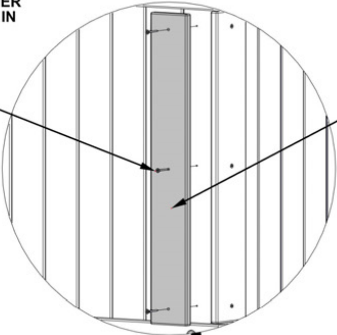
200 (x12) SCREW - 1 1/2"
