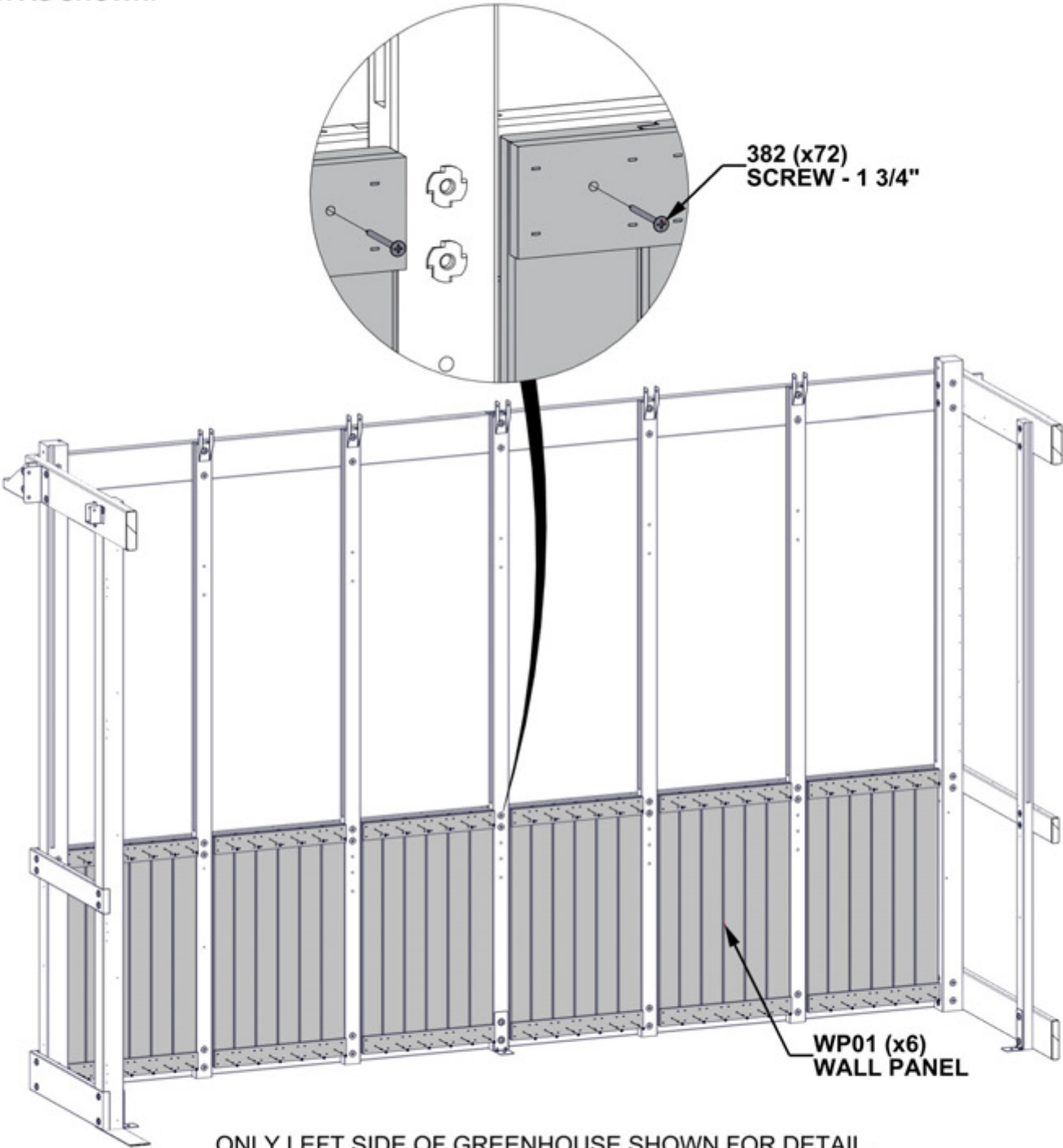
ONLY LEFT SIDE OF GREENHOUSE SHOWN FOR DETAIL.
