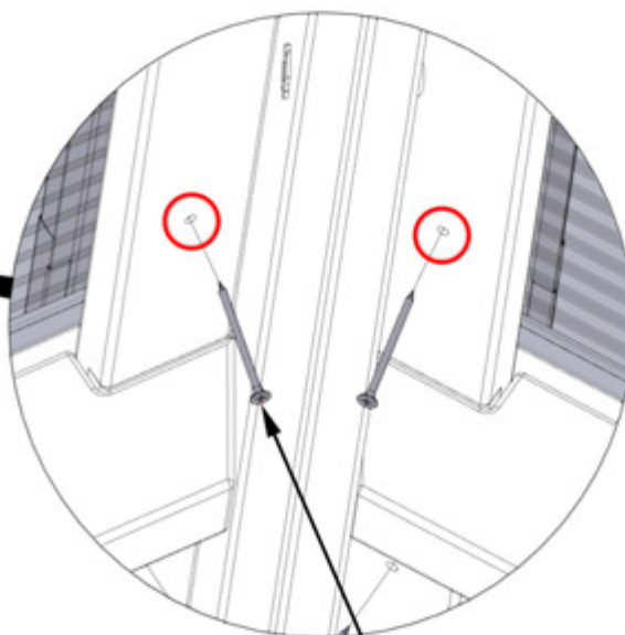
483 (x24) SCREW - 2 1/4"
