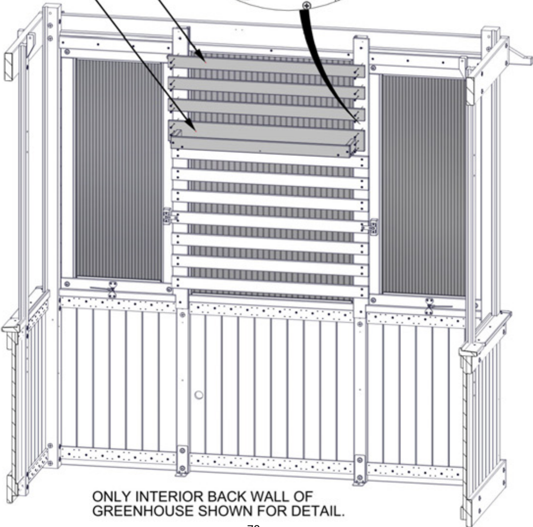
SHELF ASSEMBLY
