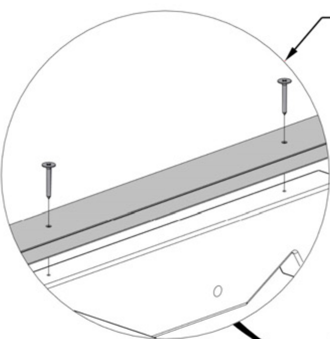
1203 (x25) SCREW - 1 1/4"
