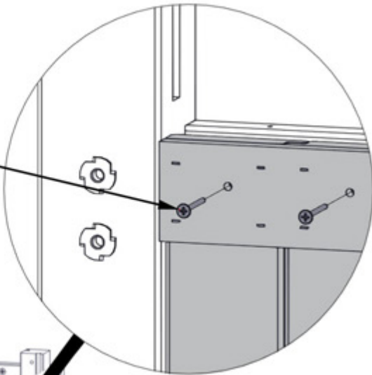
382 (x24) SCREW - 1 3/4"
