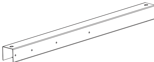
P09 Barbecue cabinet support pipe*1 40*40*555
