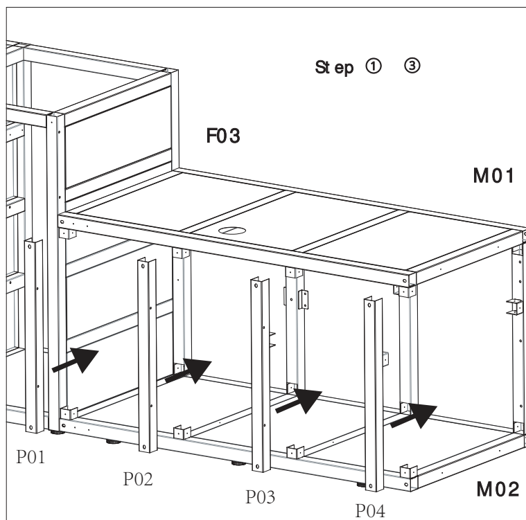
P03 Barbecue cabinet support pipe*1
