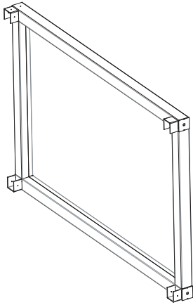
F01 Freezer right panel *1 969*635*70
