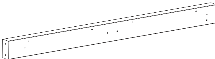
S01 Top outer frame(long) *2 100*50*1312
