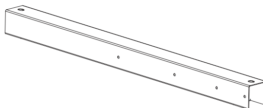
P10 Barbecue cabinet support pipe*1 40*40*555
