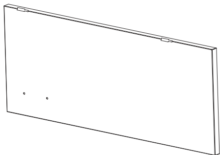
I01 Freezer right door panel *1 240*580*16
