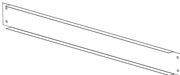
S03 Top outer frame(short) *2 100*30*1200
