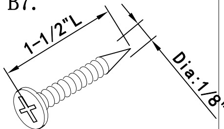
Screw
