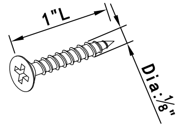
Screw
