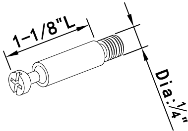
Cam-bolt
