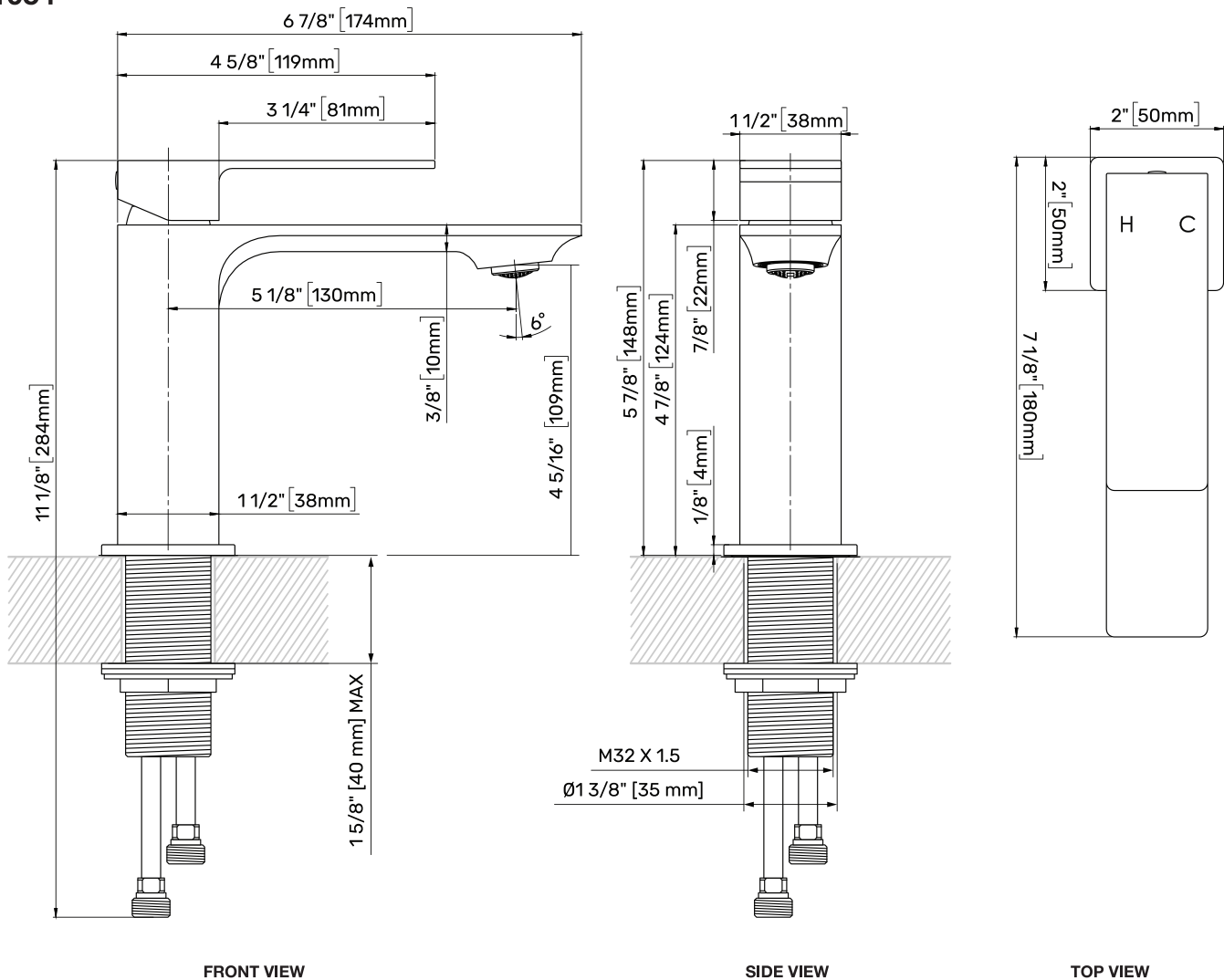
FRONT VIEW
