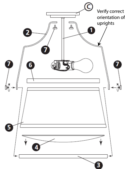
Drawing 2 – Fixture Assembly
