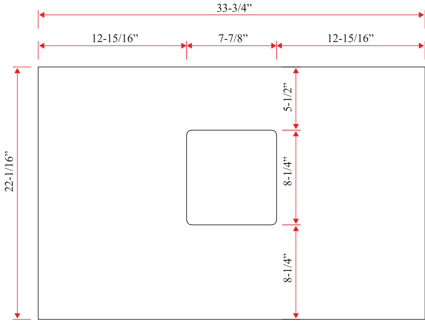
— BACKBOARD —
