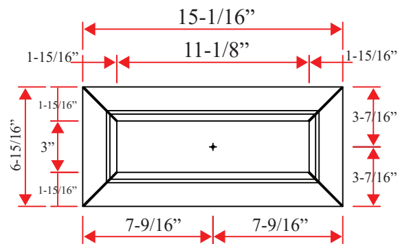
— SMALL DRAWER —
