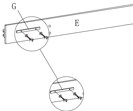
Bolt M8*60
