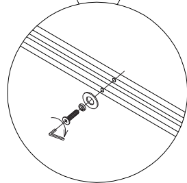
Bolt M8*60
