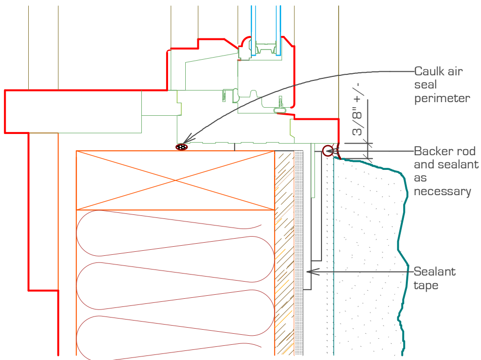
DETAIL # 10
