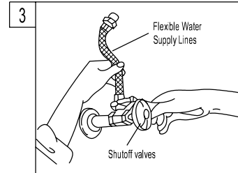
3. Connect the water supply lines. Before connecting the supply lines, apply pipe joint compound to the threads on the inlet shanks and shut off valves with an adjustable wrench.
