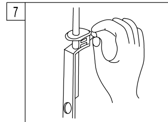
7. With lift rod in position on the faucet, insert lift rod through lift rod strap and secure with the clevis screw.
