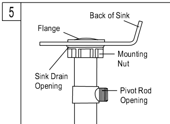
5. Install drain body up through the drain opening and reattach the flange onto drain body, holding the drain body in position with pivot rod opening facing the back of sink. Tighten the mounting nut by hand.
