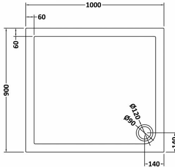
1000 x 900 RECTANGULAR TRAY
