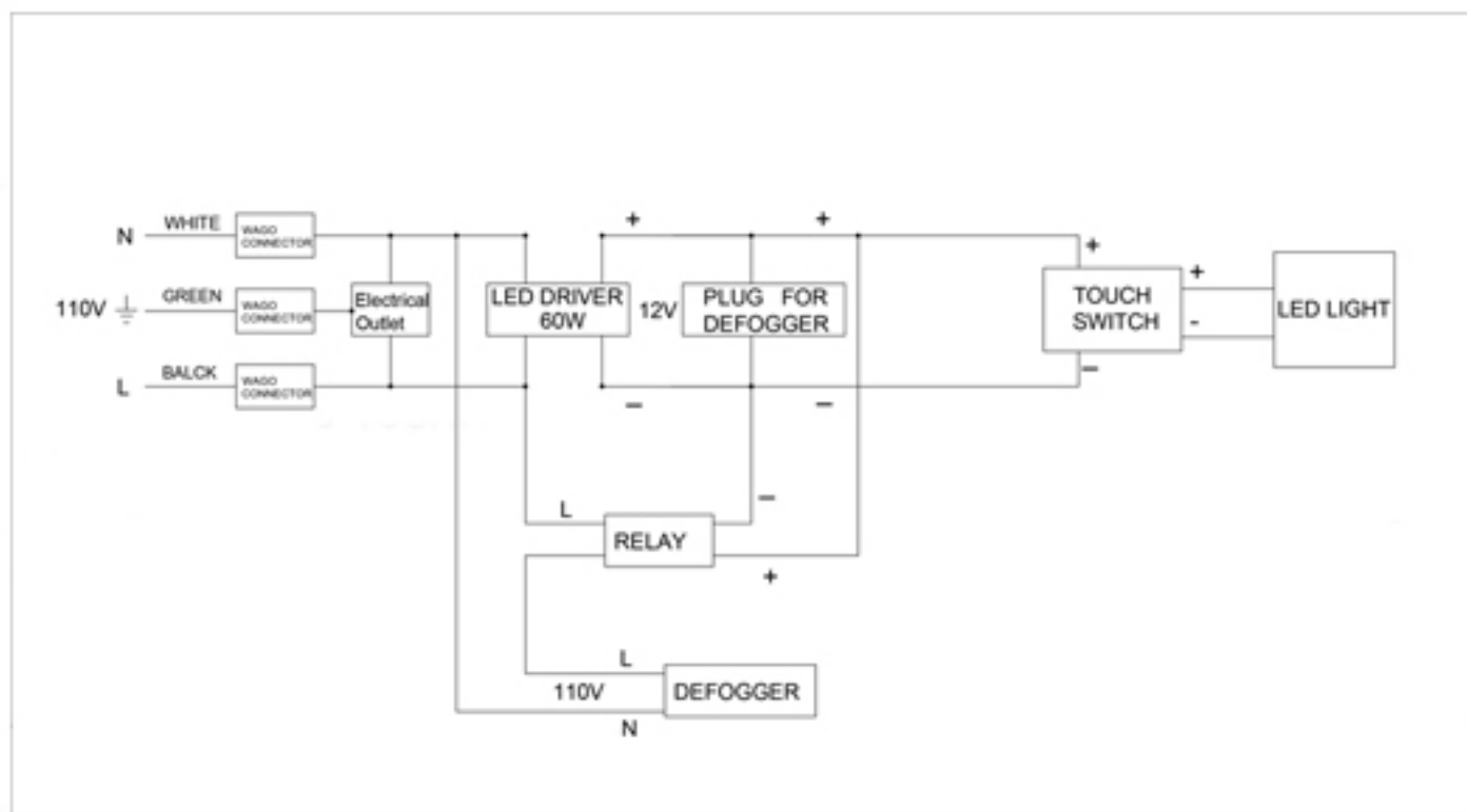
Circuit Diagram
