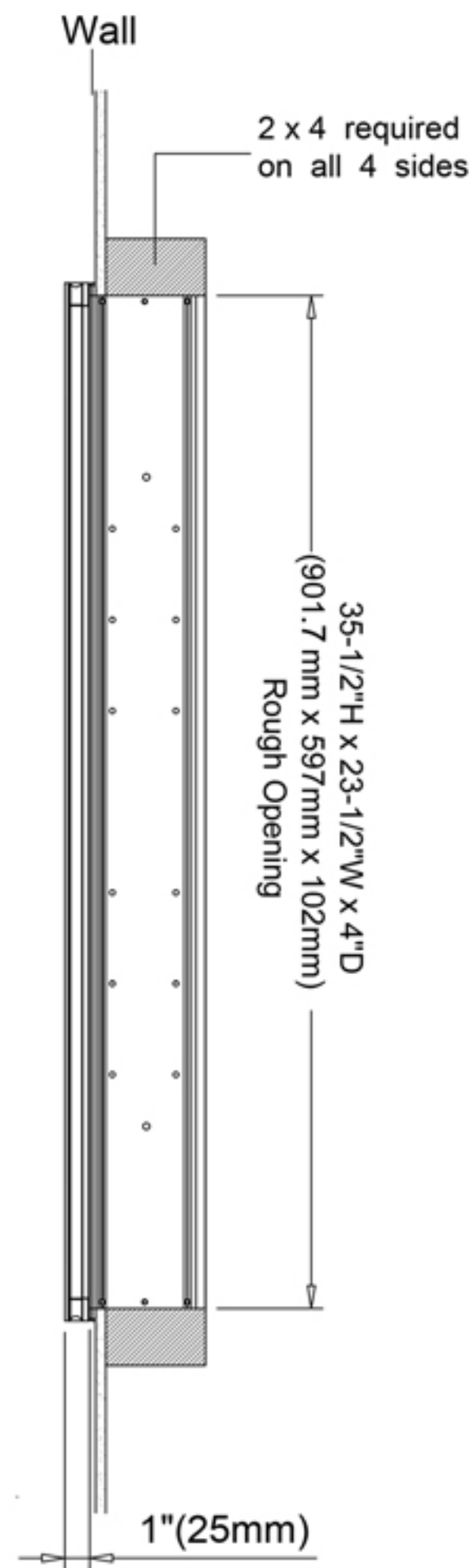
Recessed Mount
