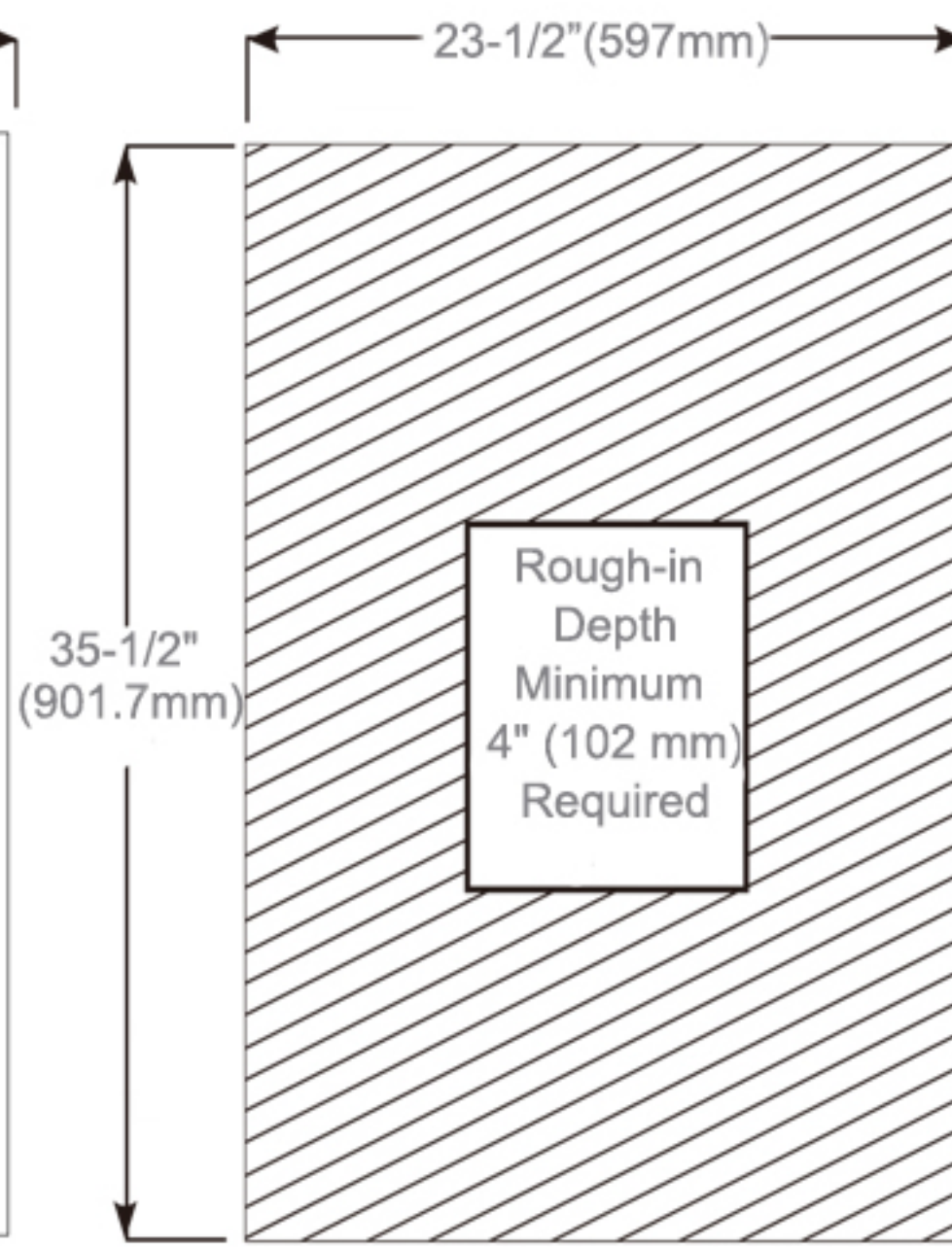
Rough-in Dimensions
