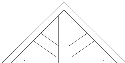
(1) WMA03 - DORMER GABLE PANEL
