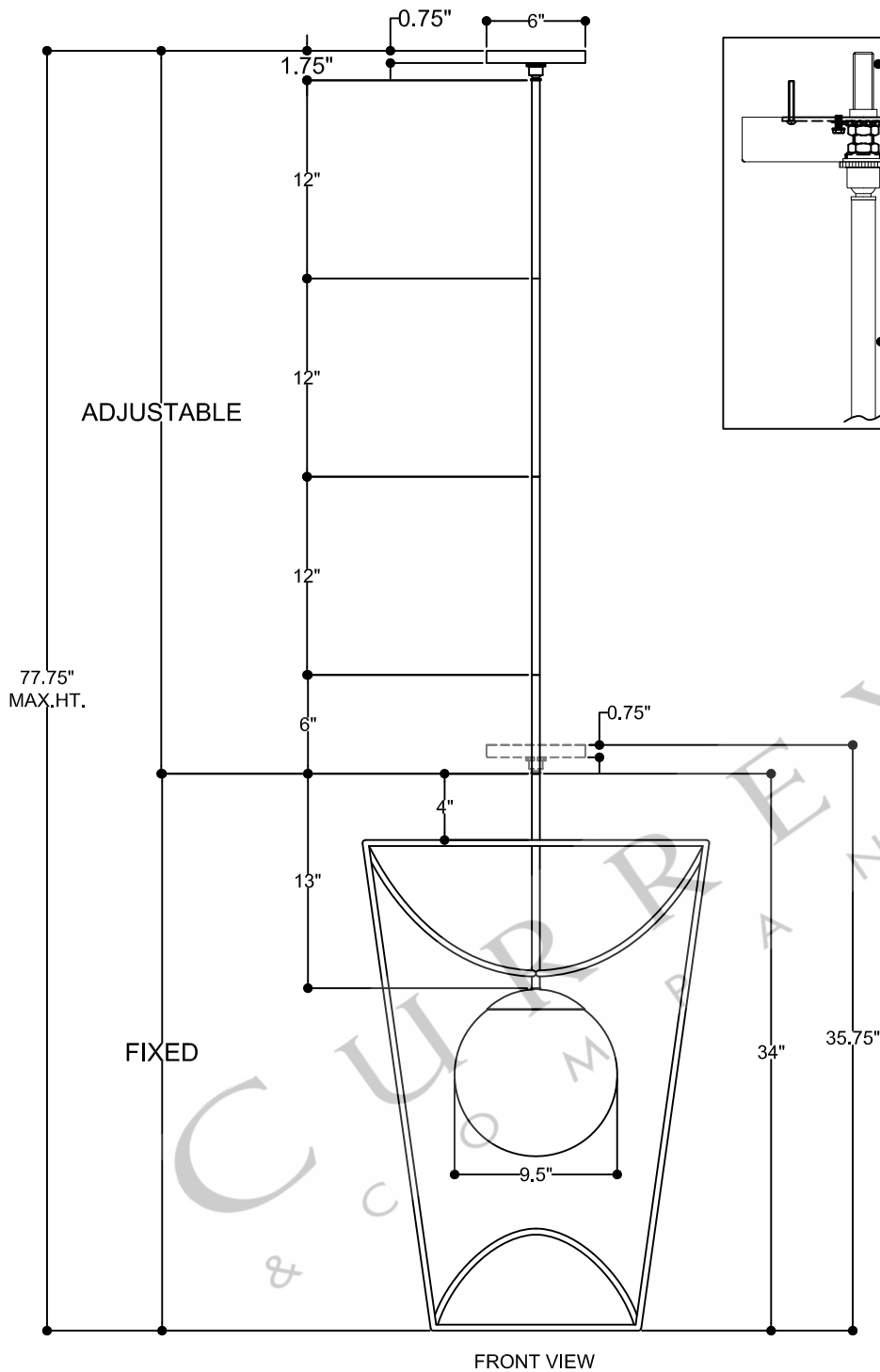
FRONT VIEW
