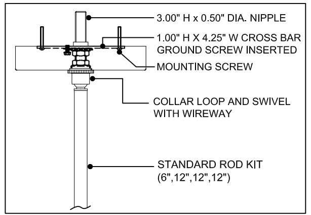
CANOPY DETAIL
