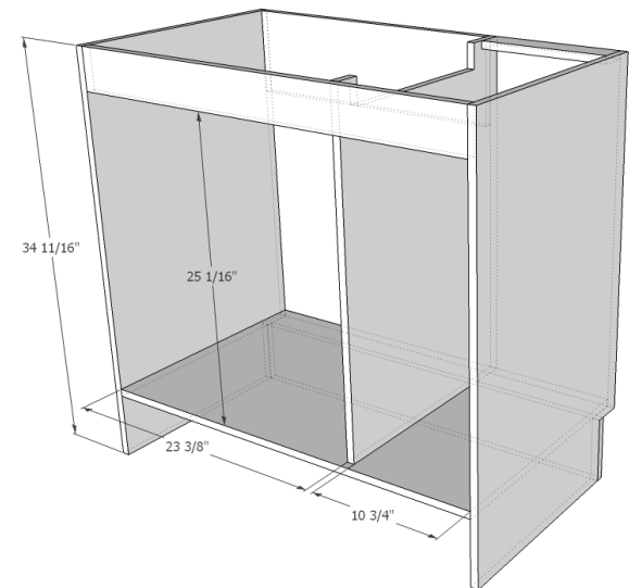
BACK DETAIL
