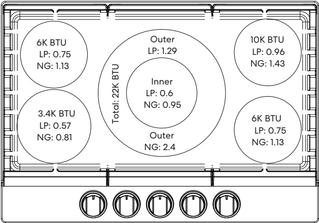
LP and NG Orifices are in size (mm)
