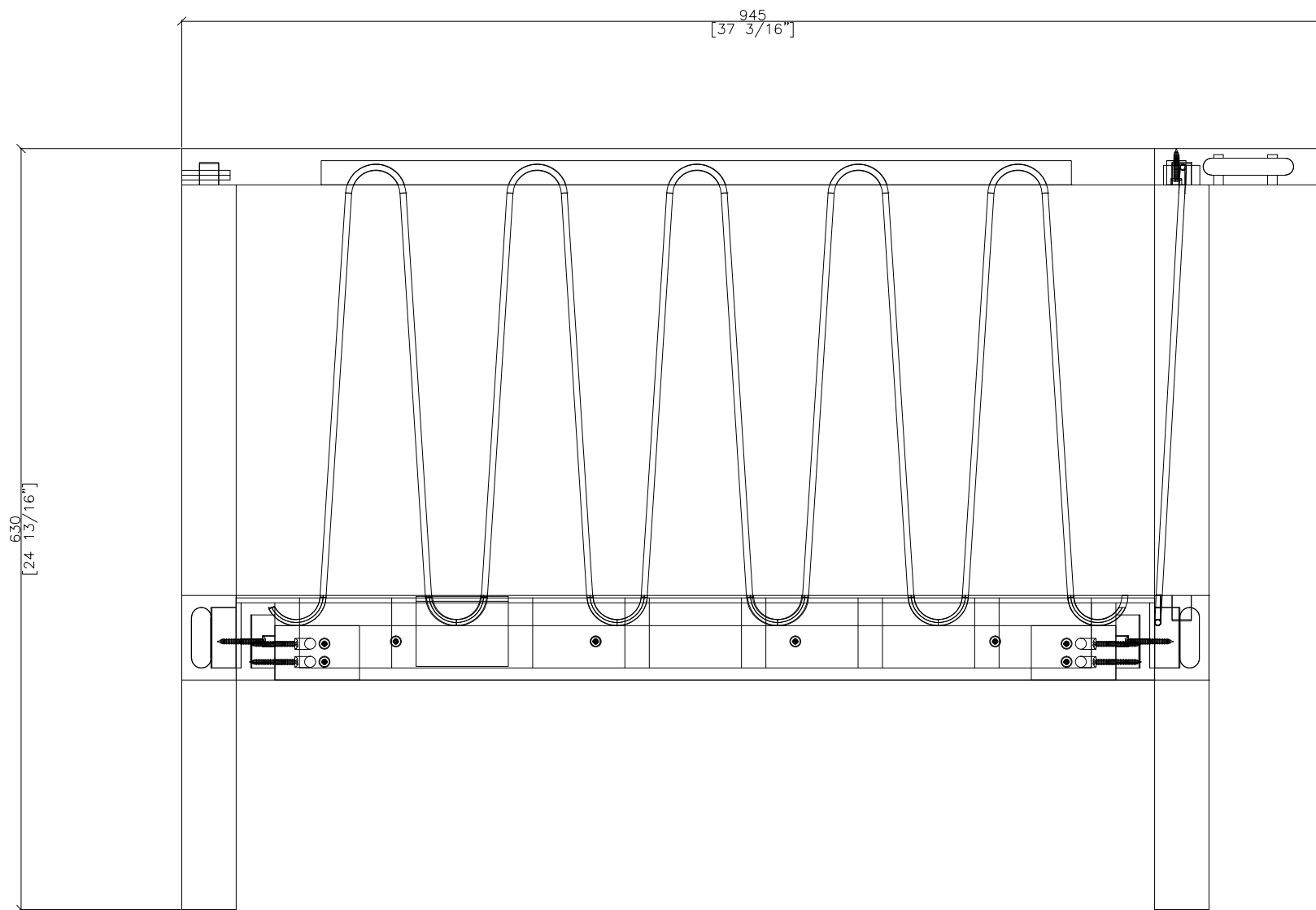
SIDE VIEW
