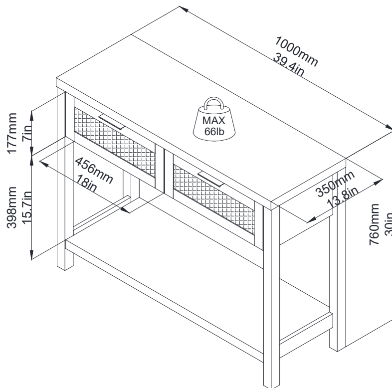
Final assmebly
