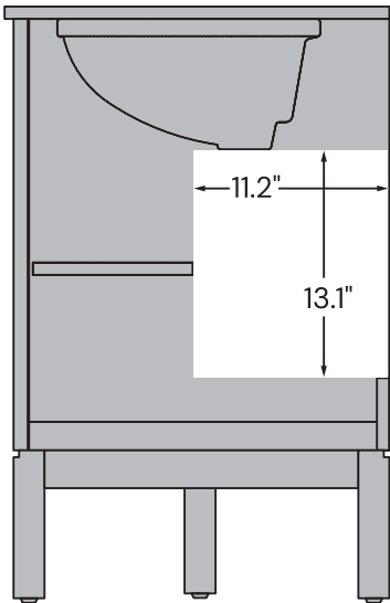
Right View
