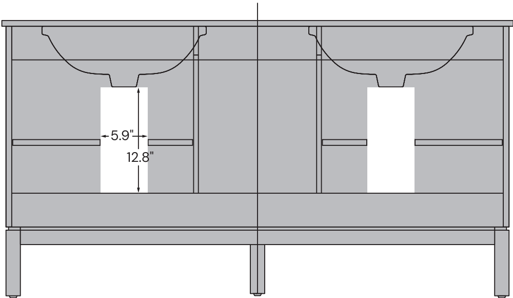
Back View
