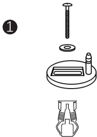
Hinge Assembly
