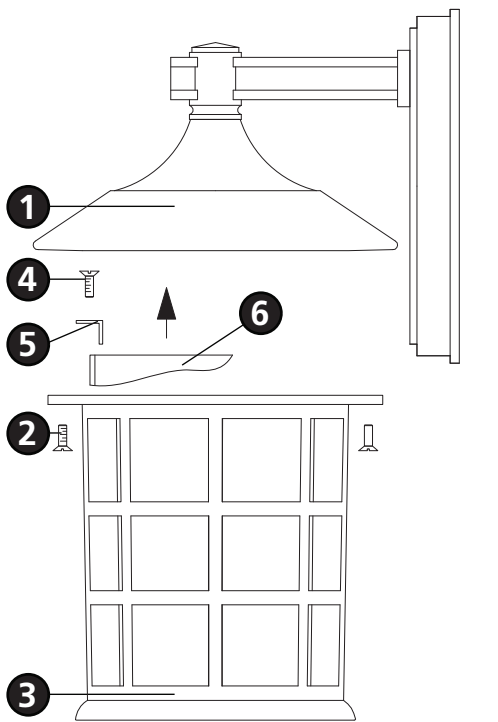
Drawing 3 - Fixture Assembly
