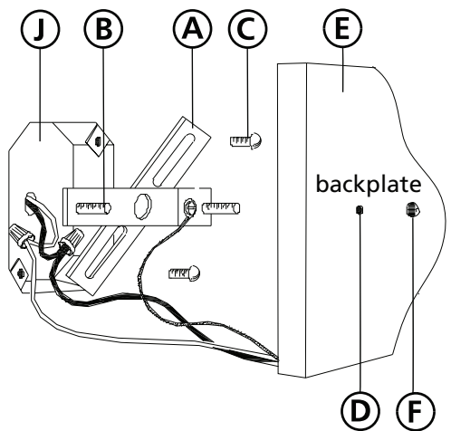
Drawing 3 - Fixture Assembly
