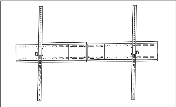
VESA MAX 1200X900(Landscape)
