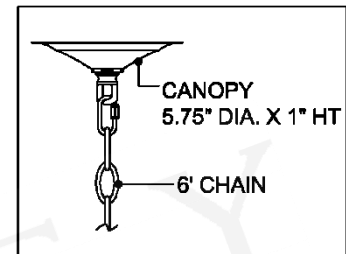
CANOPY DETAIL
