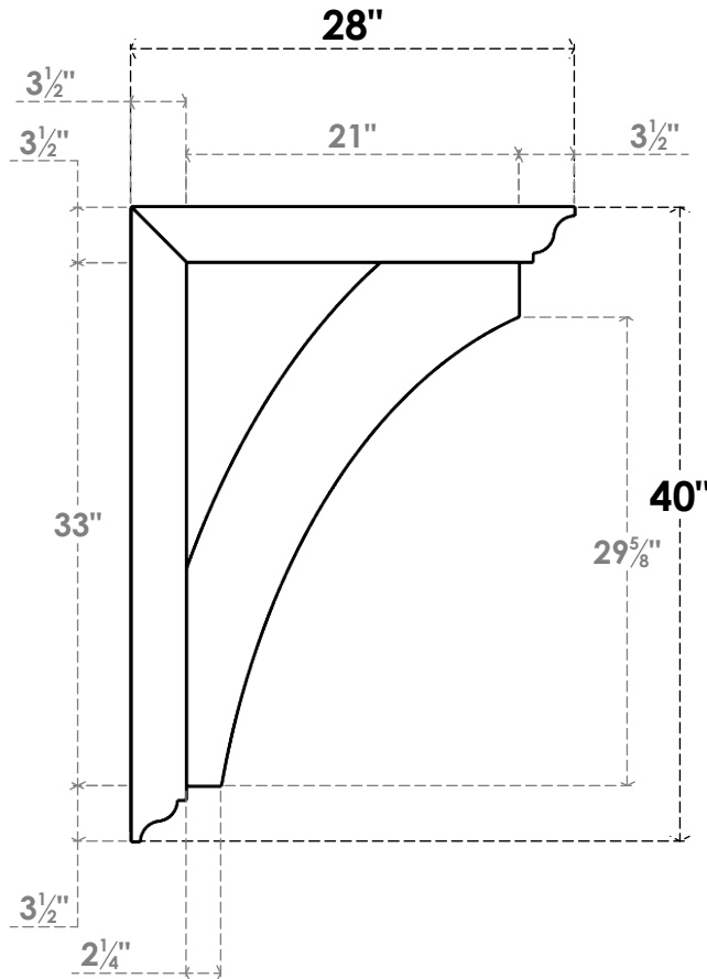
SIDE PROFILE
