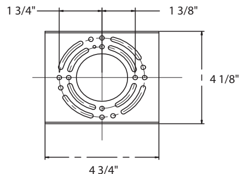
Mounting Plate Dimensions
