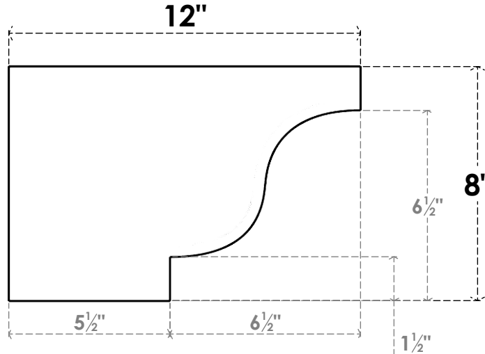
SIDE PROFILE
