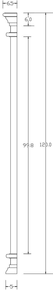
SIDE VIEW
