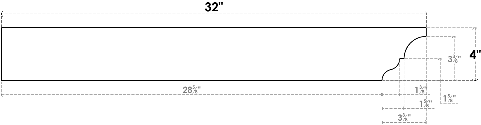
SIDE PROFILE
