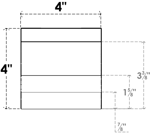
FRONT PROFILE
