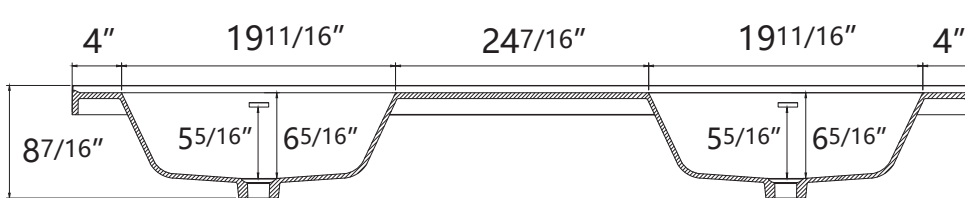
Front View
