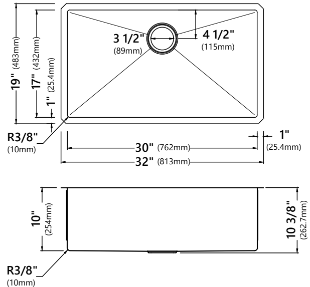
KHU100-32 32" x 17" x 10" Min Cabinet Size: 36" Matching Grid: KBG-100-32 Drain Model #: BST-1
