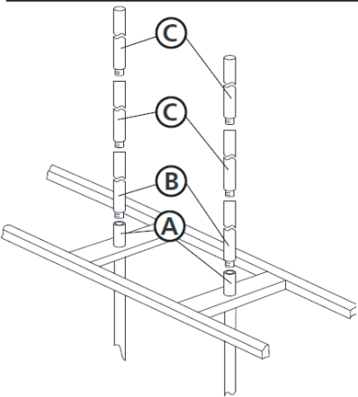
Drawing 1 – Assembly
