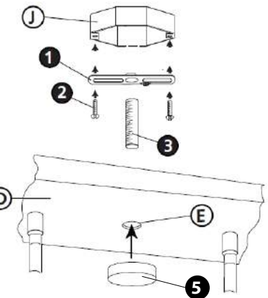
Drawing 2 – Fixture Installation
