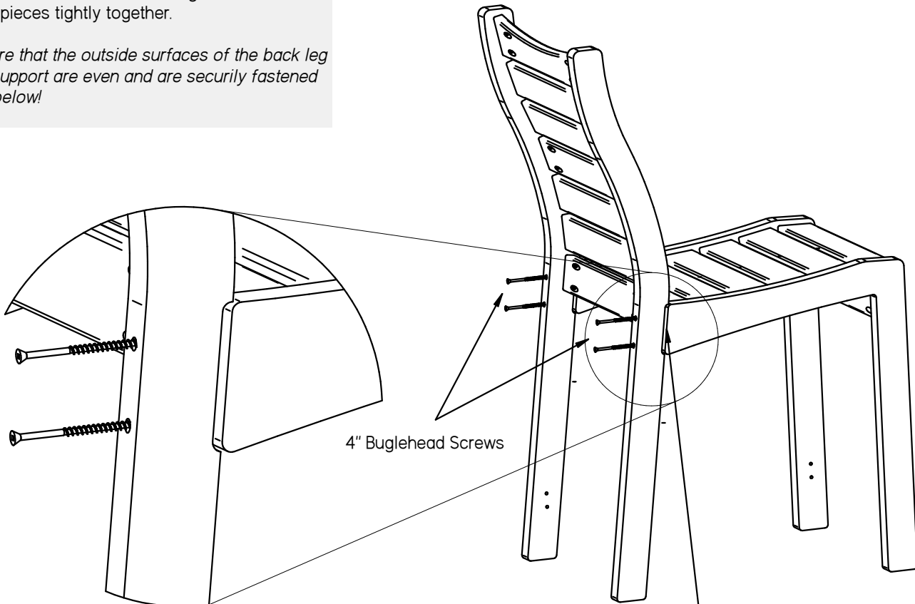
Back & Seat Assembly Detail
