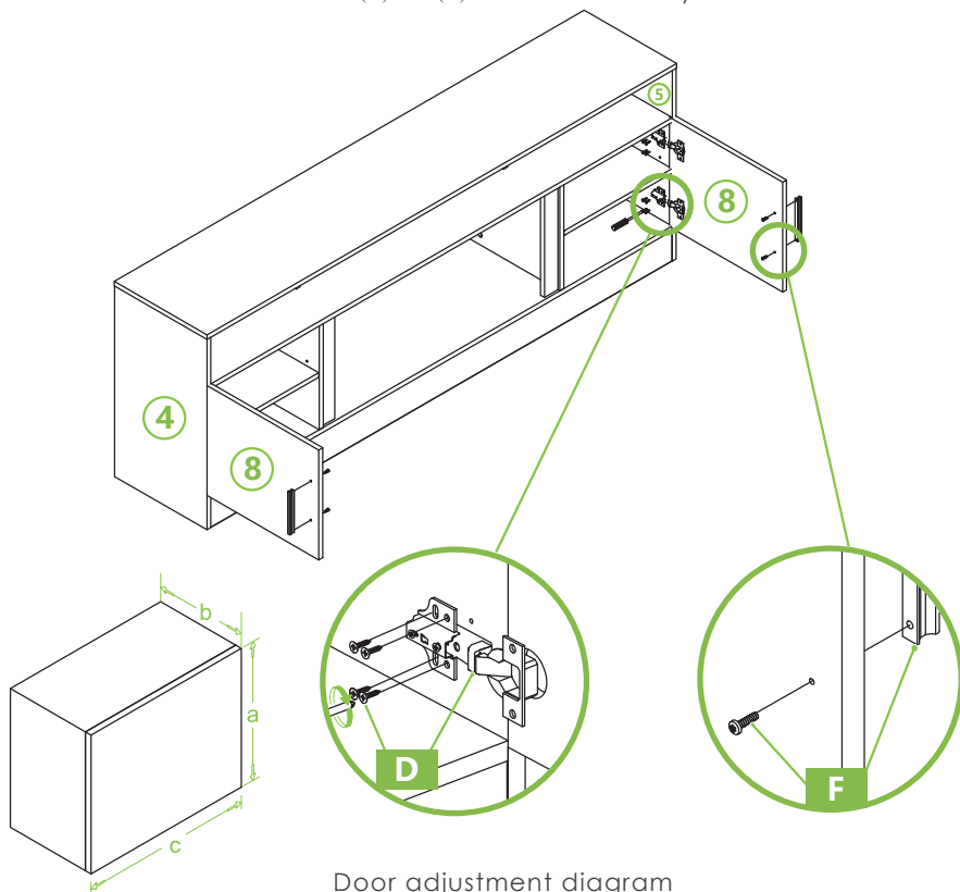
Door adjustment diagram
