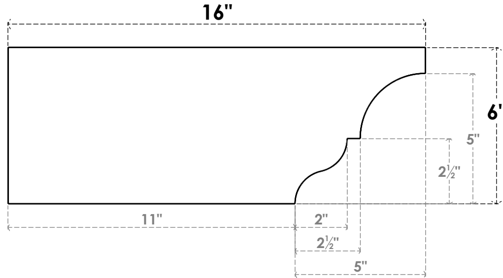
SIDE PROFILE
