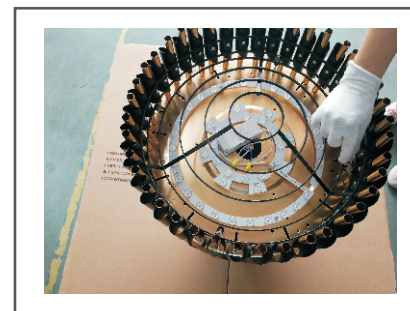
Step 4. Install the lampshade on the chassis and fix it with nuts.
