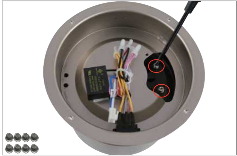
Step 3 Remove the 8 fixing screws for the fan blades.
