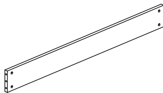
28 (930*95*15mm x1)
