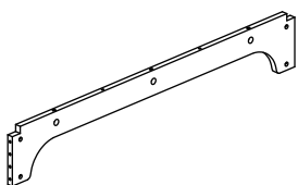
27 (930*145*15mm x1)
