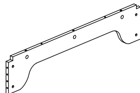
32 (800*170*15mm x1)
