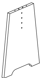
31 (400*297*18mm x2)
