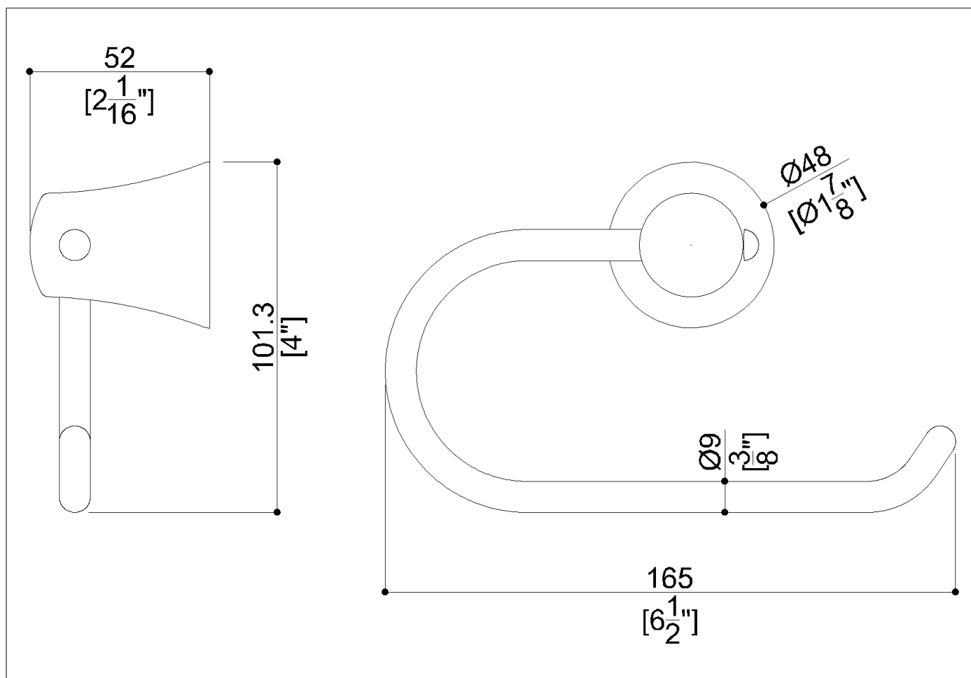
Column Roll Paper Holder, Polished
