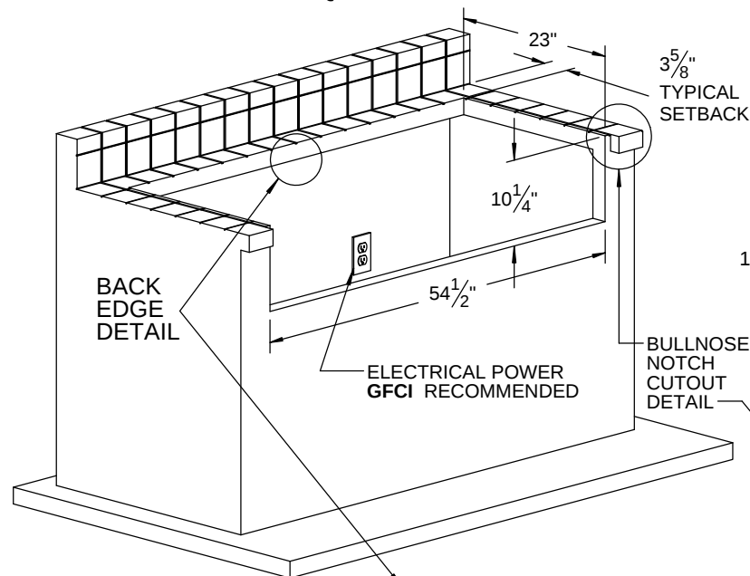
TYPICAL ALXE-56 BFG INSTALLATION
