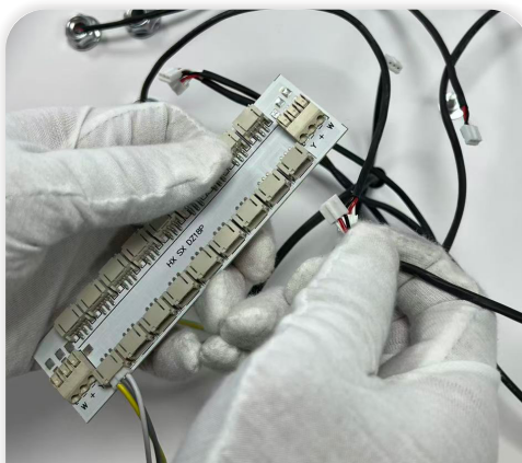
11 Insert the lamp holder wire into the terminal block.
