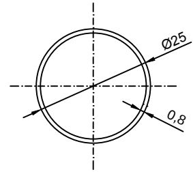
TUBE DETAIL
