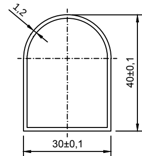
PROFILE DETAIL
