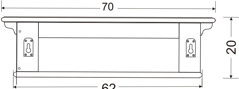
Back view
