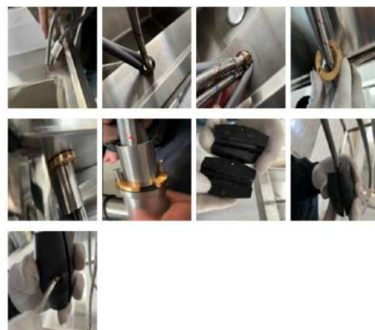
Step 7: Sink installation completed
