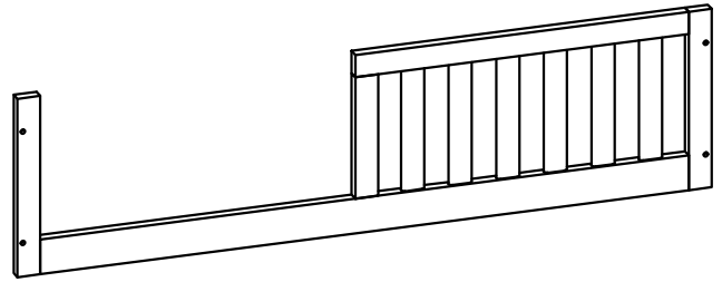
Guard Rail - 1pc
