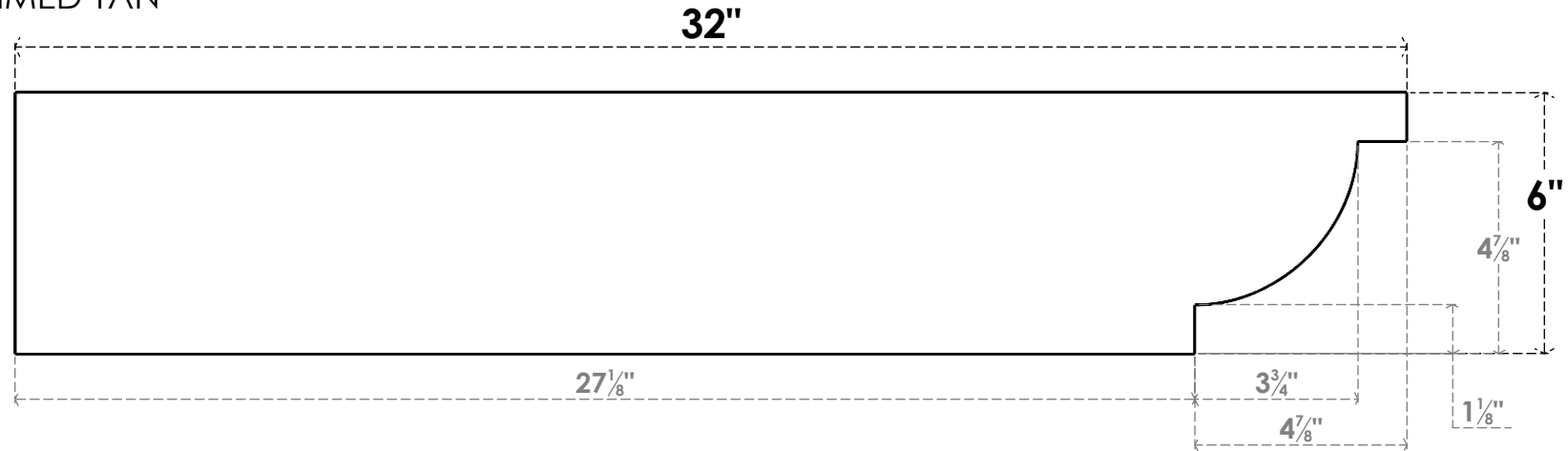
SIDE PROFILE
