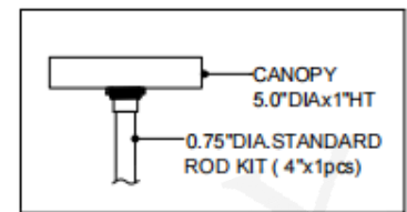
CANOPY DETAIL
