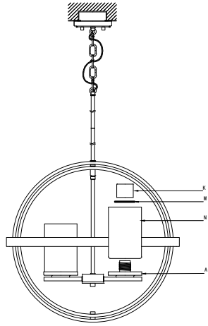
Step 12-Use K to secure M and N to A.
