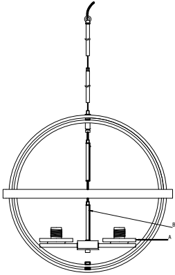
Step 1-Connect B to A.
