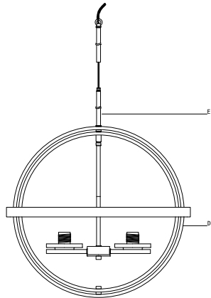
Step 4-Connect E to D.
