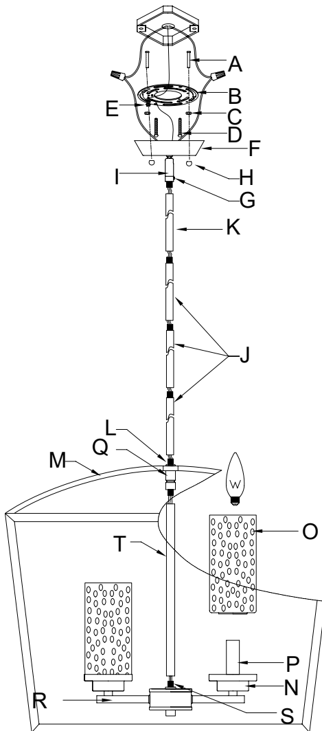
How to Identify the Fixture's Wires
