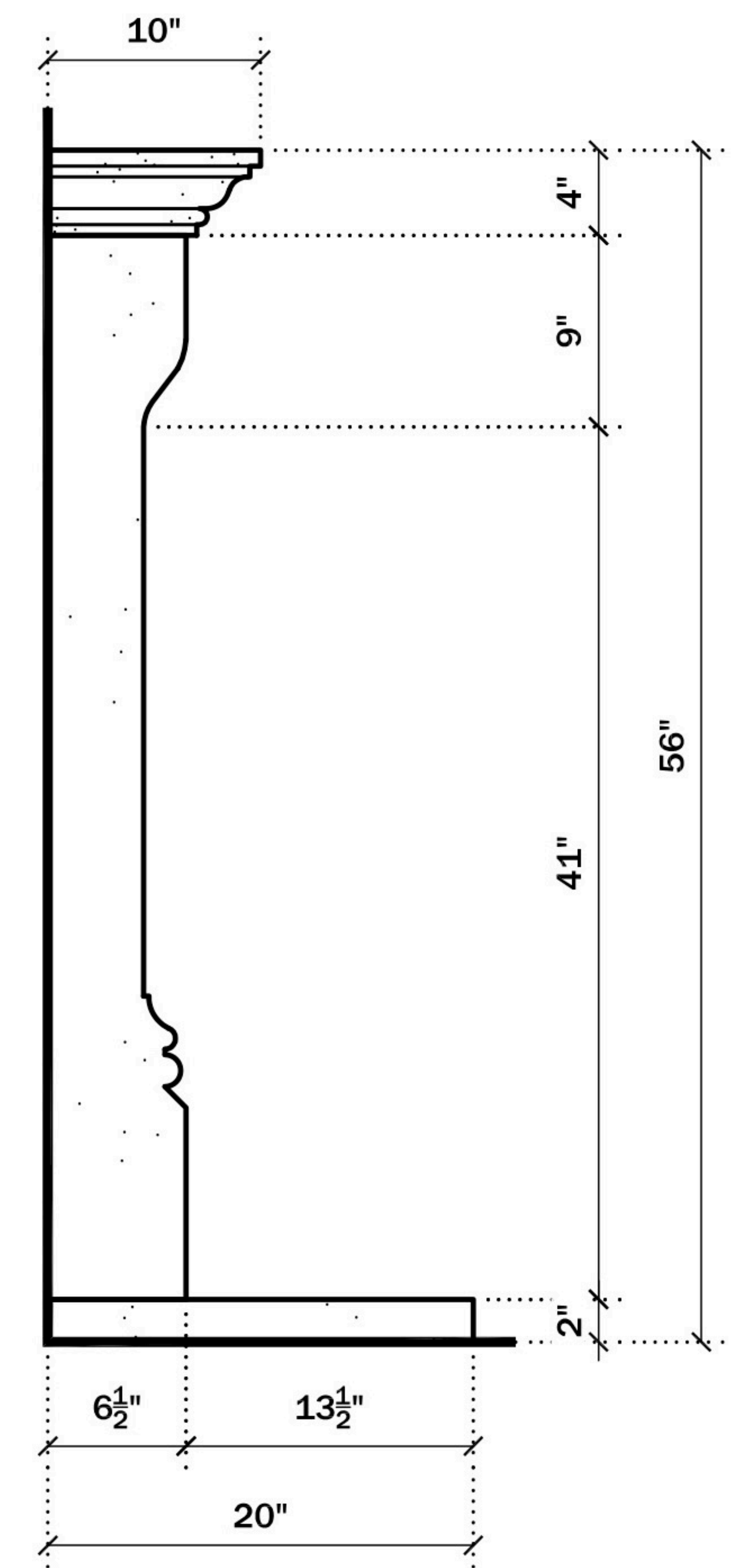
SIDE VIEW
