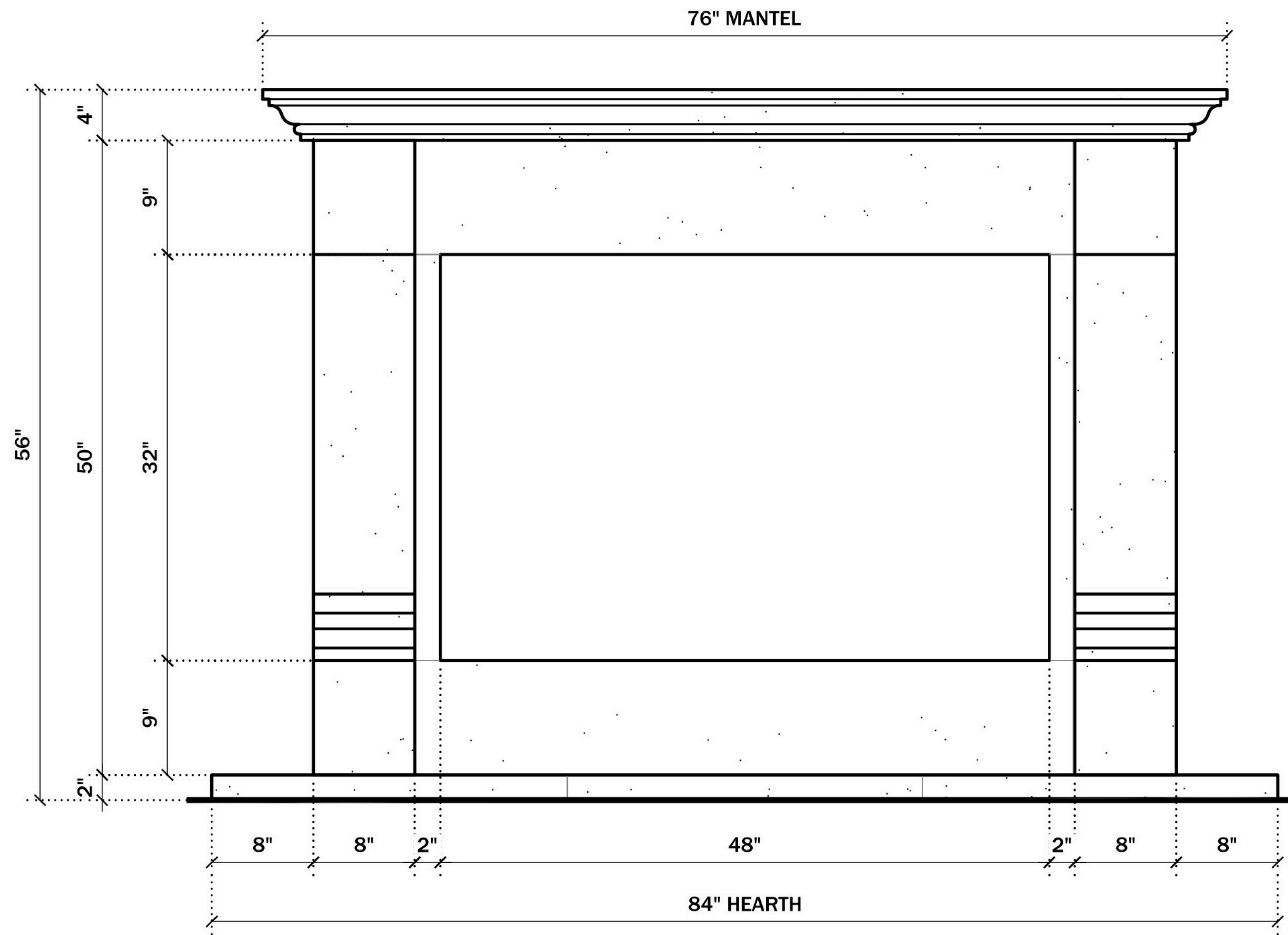
FRONT ELEVATION
