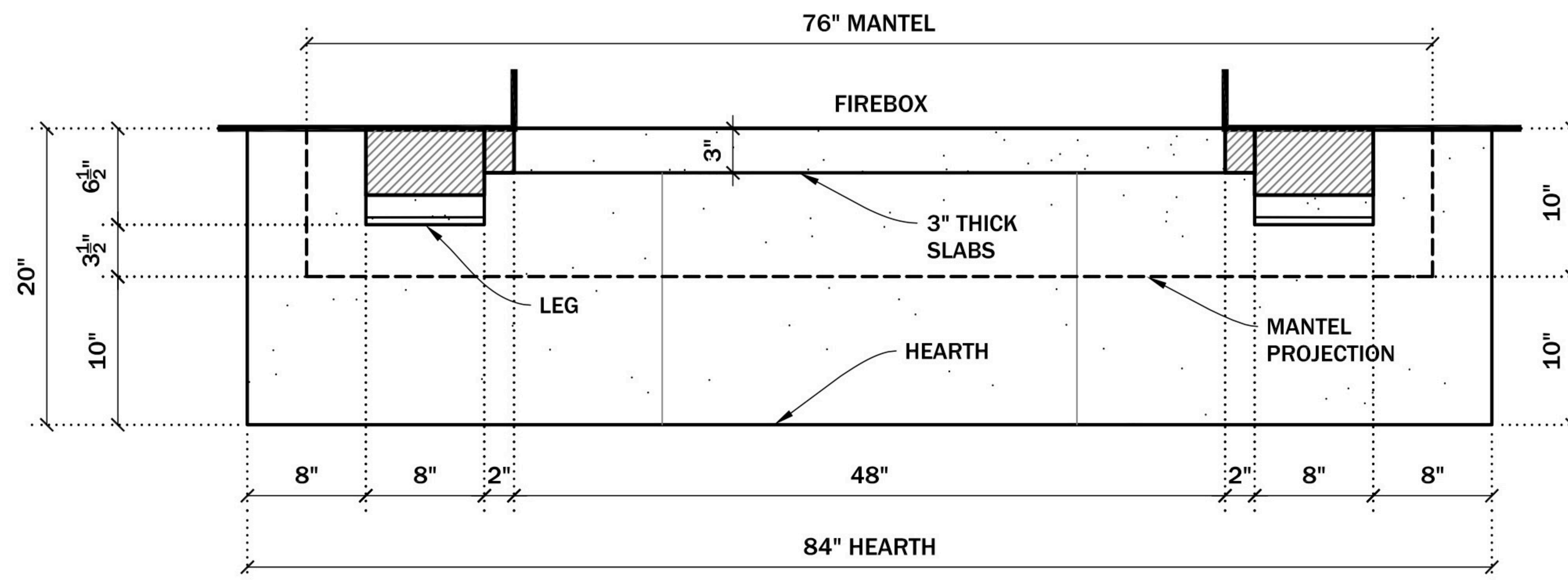
PLAN VIEW
