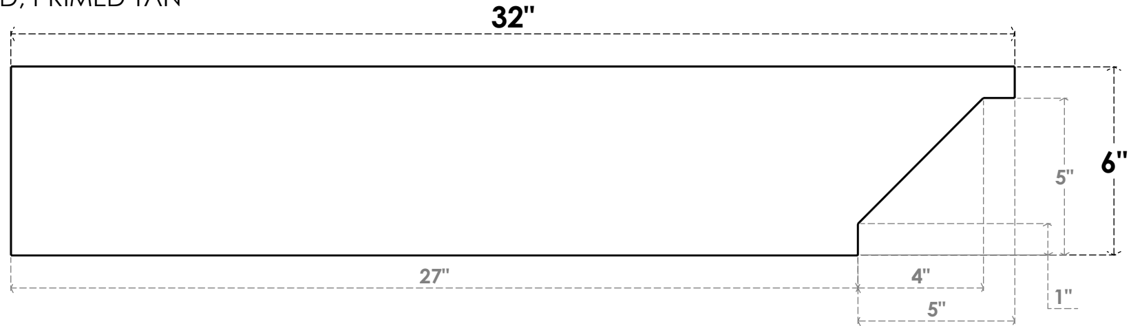
SIDE PROFILE
